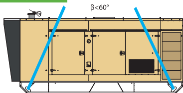
GV121 - GV151 - GV201 - GV301 MOVABLE WITH WEB SLINGS
