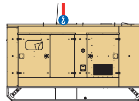
GV151 - GV201 -> TOP ROOF DOOR CENTRAL LIFTING POINT
